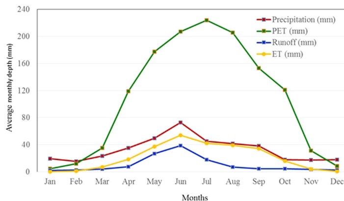
Figure 2. Average monthly values of water balance components in the Oldman River Basin (1953–2001). Precipitation and runoff are based on measured values; PET is estimated using Penman-Monteith method, and actual evapotranspiration (ET) is predicted using the conceptual model developed in this study (introduced later in section 5.2).
