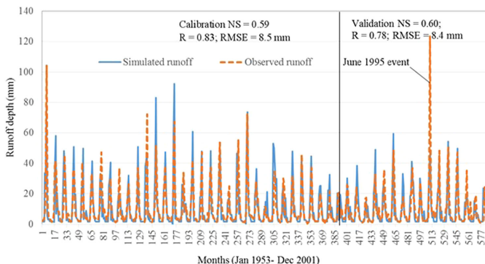
Figure 5. Observed and simulated monthly runoff at the outlet of the OMRB, Alberta, Canada. The developed conceptual model performs well in predicting the monthly runoff values with Nash-Sutcliffe value of 0.60 and correlation coefficient of 0.78.
