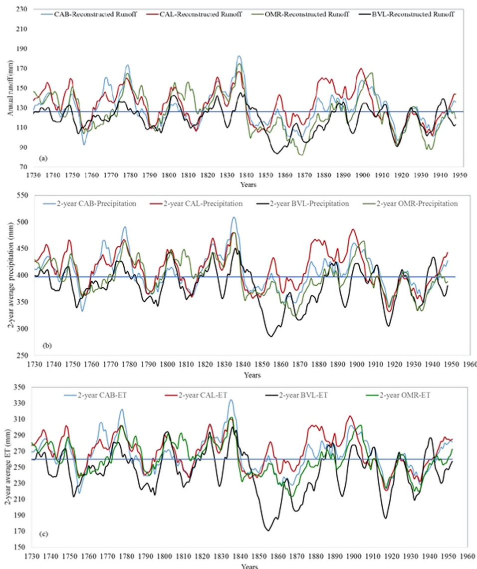
Figure 6. Five year running average of (a) reconstructed annual runoff, (b) 2 year average precipitation, and (c) 2 year average evapotranspiration for the OMRB. The horizontal line shows the mean value based on the instrumental period (1955–2001).
