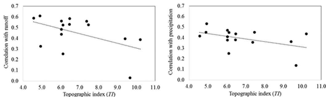
Figure 4. Topographic index and correlation between TRCs and hydrological variables at various sites in the OMRB. There is obvious trends showing that the higher the topographic index values (potentially wetter sites), the lower the correlation coefficient values between TRCs and hydrological variables.
